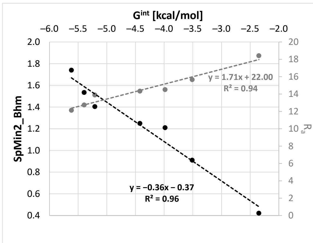
Figure 7. Exemplary regressions documenting the quality of the linear relationships between the COSMO-RS-DARE interaction parameter, G^{\text{int}} , and molecular descriptors SpMin2_Bhm (Burden modified eigenvalue descriptor) and R_a (distance between solute and solvent in the Hansen solubility space).
