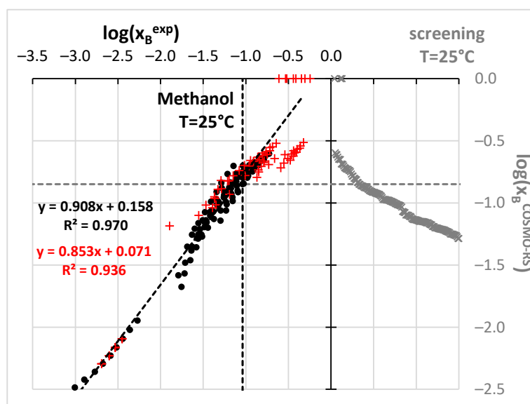
Figure 2. Results of benzamide solubility measurements and computations. All experimental points marked as black circles were taken from the literature while new measurements are presented as red pluses. Computed solubility values are presented in gray color. Dashed lines stand for best solubility values estimated so far at room temperature.
