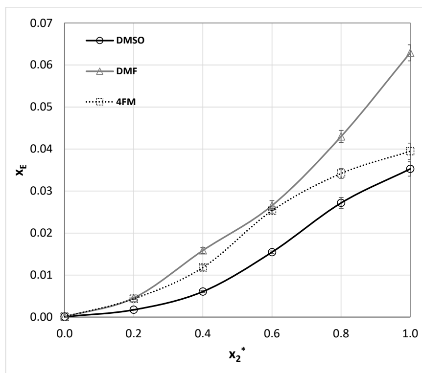
Figure 7. The results of ethenzamide solubility measurements (molar fraction, x_E ) at room temperature in aqueous DMSO, DMF, and 4FM mixtures ( x_2^* stands for the organic component mole fraction in the binary solvent). The error bars denote standard deviation values ( n = 3 ).
