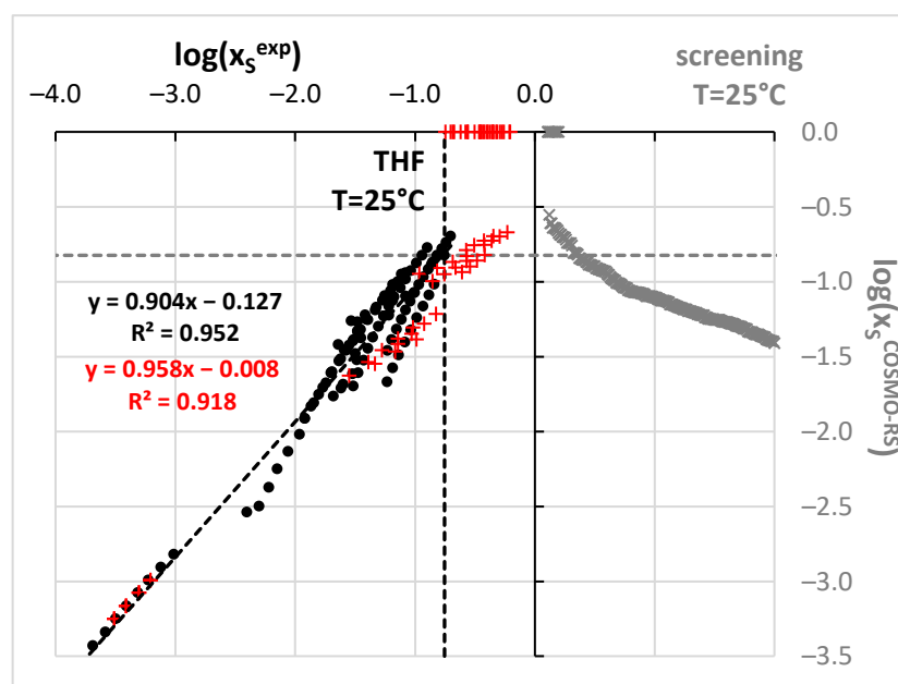
Figure 5. Results of salicylamide solubility measurements and computations. Notation is the same as in Figure 2.
