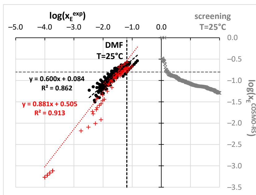
Figure 9. Results of ethenzamide solubility measurements and computations. Notation is the same as in Figure 2.
