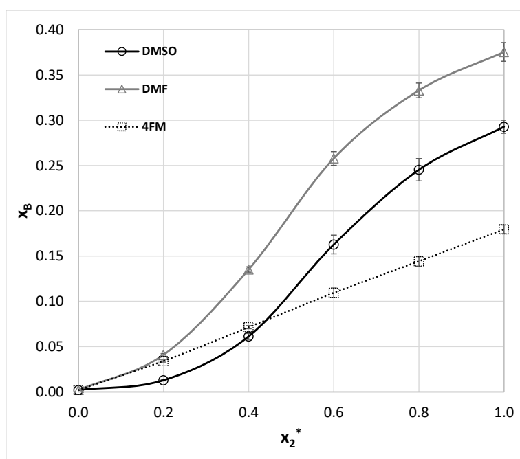
Figure 3. The results of benzamide solubility measurements (molar fraction, x_B ) at room temperature in aqueous DMSO, DMF, and 4FM mixtures ( x_2^* stands for the organic component mole fraction in the binary solvent). The error bars denote standard deviation values ( n = 3 ).
