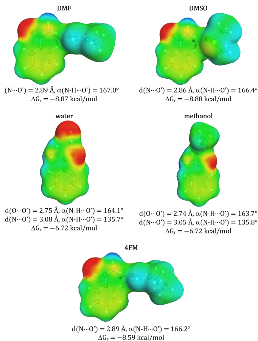
Figure 1. Structural and thermodynamic characteristics of selected solute-solvent contacts of benzamide. The affinity measure ( \Delta G_r ) represents concentration-independent value associated with activity constant of the corresponding reaction of pair formation at room temperature. Prime denotes atoms belonging to solvent molecules.
