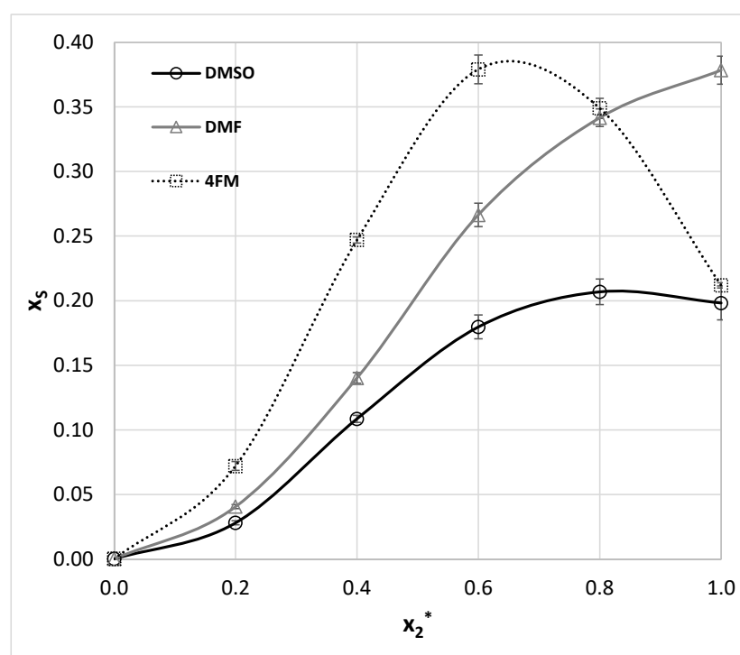
Figure 4. The results of salicylamide solubility measurements (molar fraction, x_S ) at room temperature in aqueous DMSO, DMF, and 4FM mixtures ( x_2^* stands for the organic component mole fraction in the binary solvent). The error bars denote standard deviation values ( n = 3 ).
