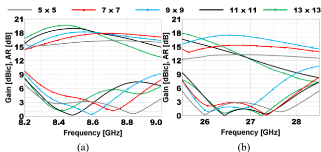
Fig. 2. Simulated maximum gain and axial ratio for five different PRS configuration (a) X-band antenna (b) Ka-band antenna
