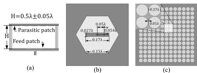
Fig. 1. Geometry of the antenna with superstrate layer side view (a), radiating element (b) and exemplary PRS structure (c)
