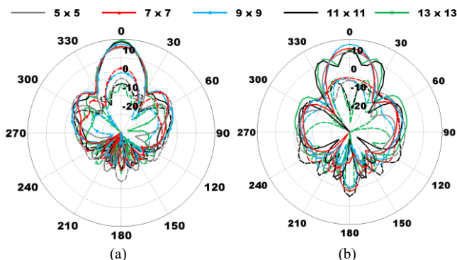
Fig. 3. Simulated radiation patterns for five different PRS configuration \Phi = 0^\circ plane (a) at 8.4 GHz (b) at 26.5 GHz
