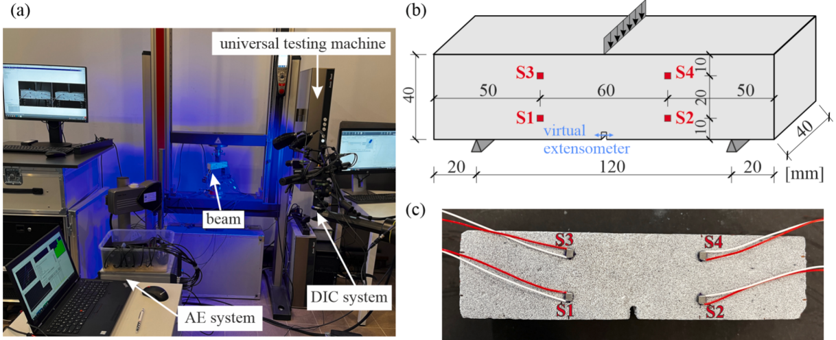
Fig. 1. (a) Experimental setup for integrated AE and DIC measurements; (b) the geometry of the beams and the location of PZT sensors; (c) the photograph of the front side of the beam before bending test.
