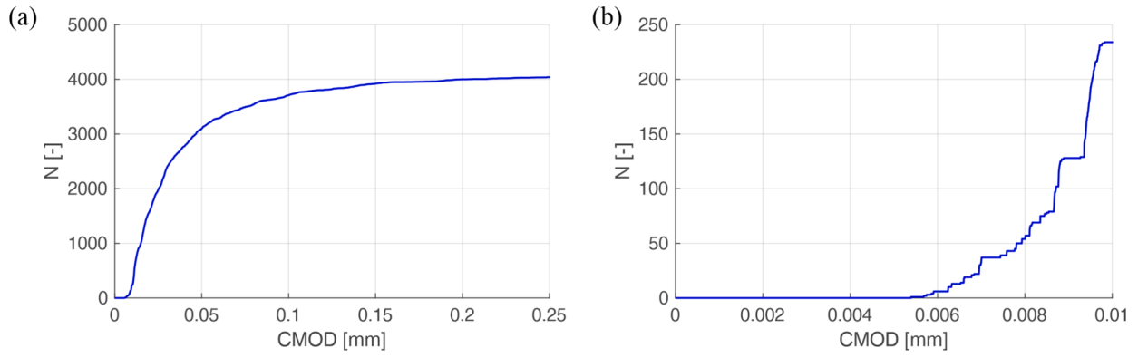
Fig. 11. The broken contacts in the specimen versus CMOD (a) whole test and (b) zoom in pre-peak part.
