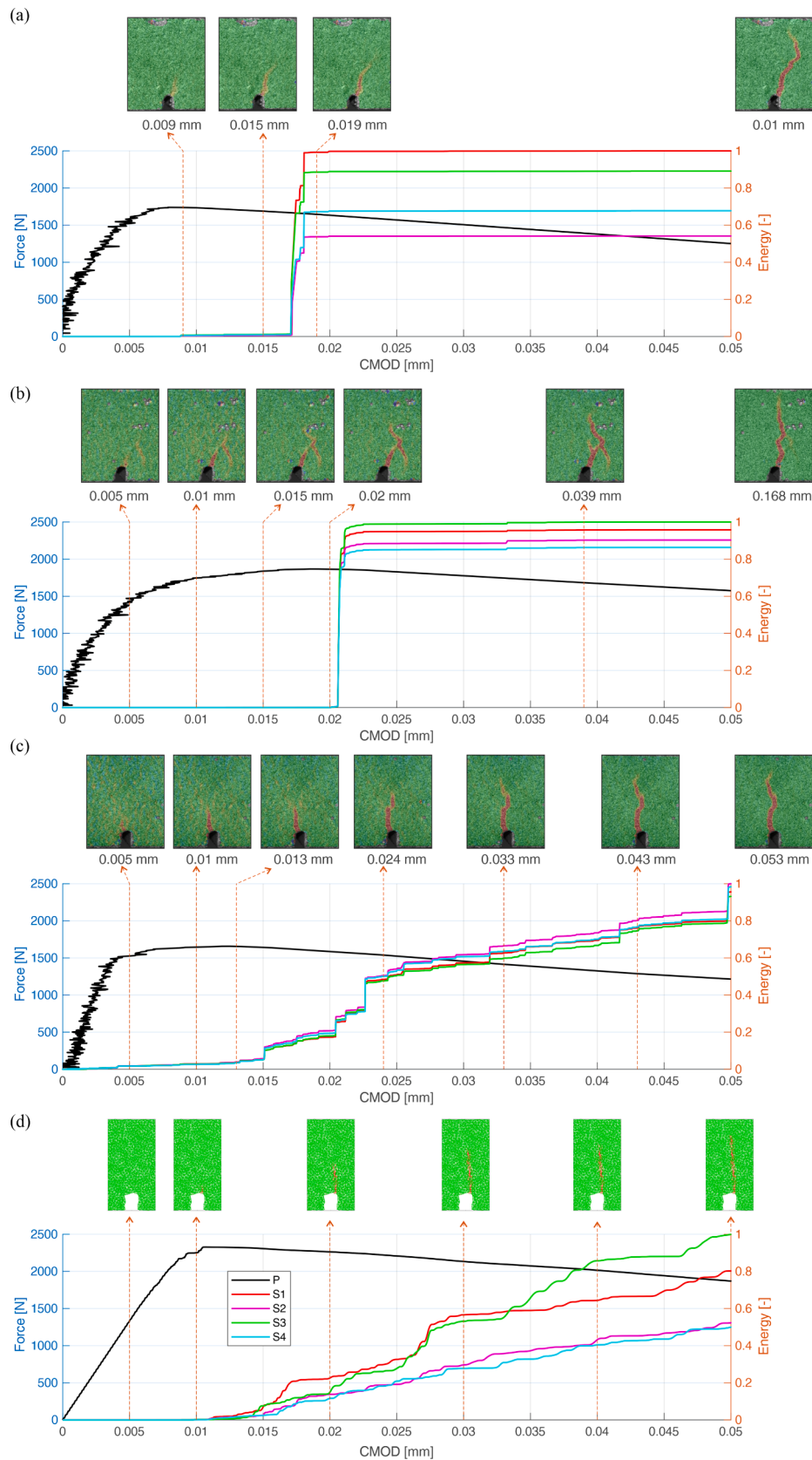
Fig. 14. Integrated results: force and cumulative energy–CMOD curves with images of cracking development: (a) beam #1, (b) beam #2, (c) beam #3, (d) numerical 3D DEM beam model.
