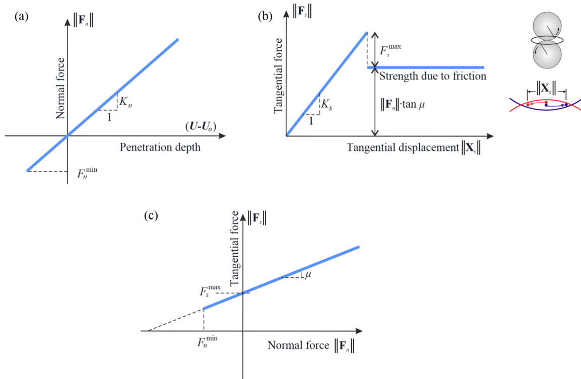
Fig. 2. Mechanical response of DEM: (a) normal contact model, (b) tangential contact model and (c) modified Mohr-Coulomb model [44,45].
