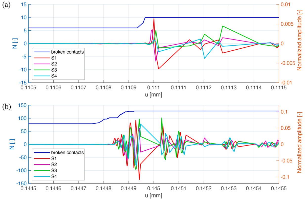
Fig. 13. The broken contacts in the specimen versus displacements, together with signal registered by all the sensors S1-S4 at selected displacements values: (a) 0.1105 mm to 0.1115 mm; (b) 0.1445 mm to 0.1455 mm.
