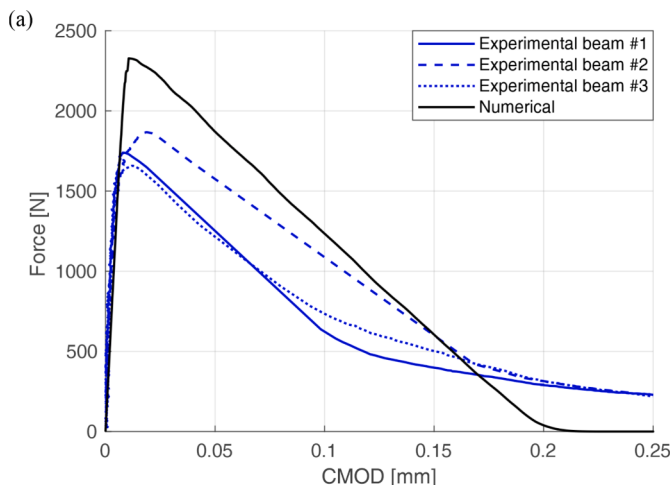
Fig. 4. Results from bending: (a) force-CMOD curves and (b) force-displacement curves for experimental beams #1–3 and numerical beam.
