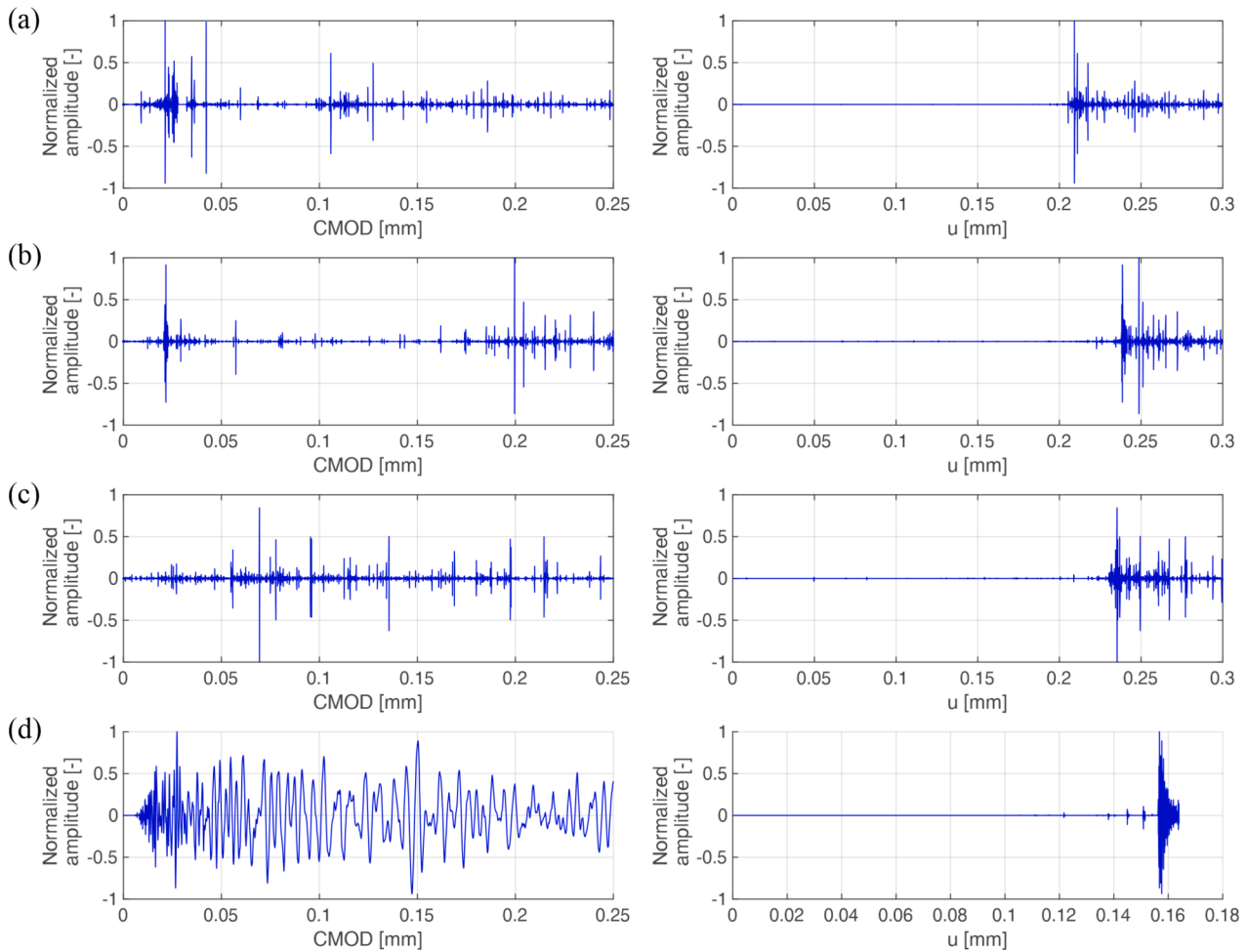
Fig. 8. Elastic wave signals acquired during experiments and in numerical simulations in the CMOD domain (first column) and in the displacement domain (second column): (a) beam #1, (b) beam #2, (c) beam #3, (d) numerical 3D DEM beam model.
