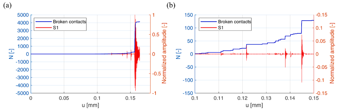
Fig. 12. The broken contacts in the specimen versus displacements, together with signal registered by sensor S1: (a) whole test and (b) zoom in pre-peak part.
