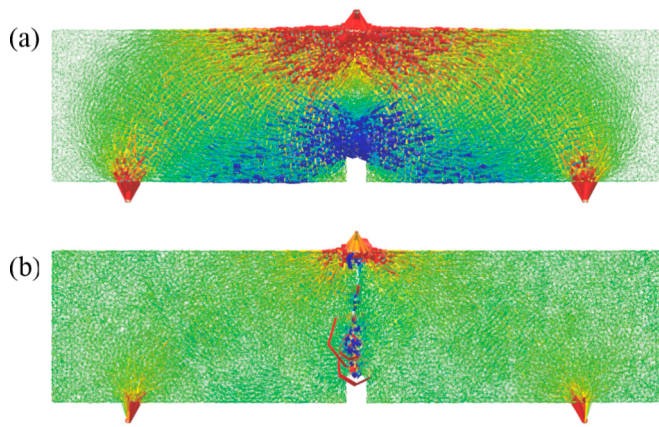
Fig. 6. Distribution of forces (red colour – compression, blue colour – tension) in 3D DEM model of concrete beam for different values of CMOD: (a) 0.008 mm, (b) 0.1 mm.
