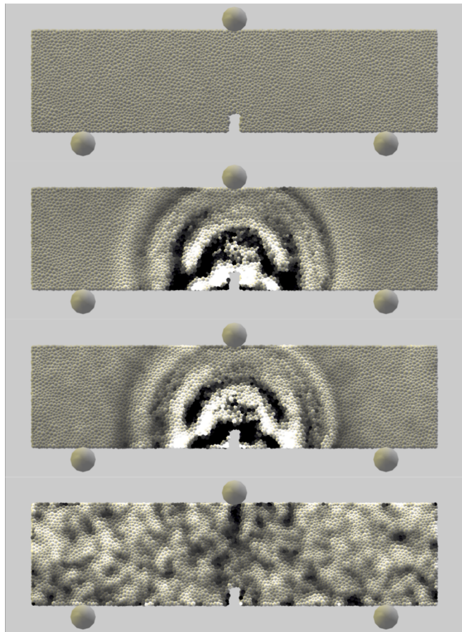
Fig. 7. Snapshots of acceleration field in the 3D DEM model.
