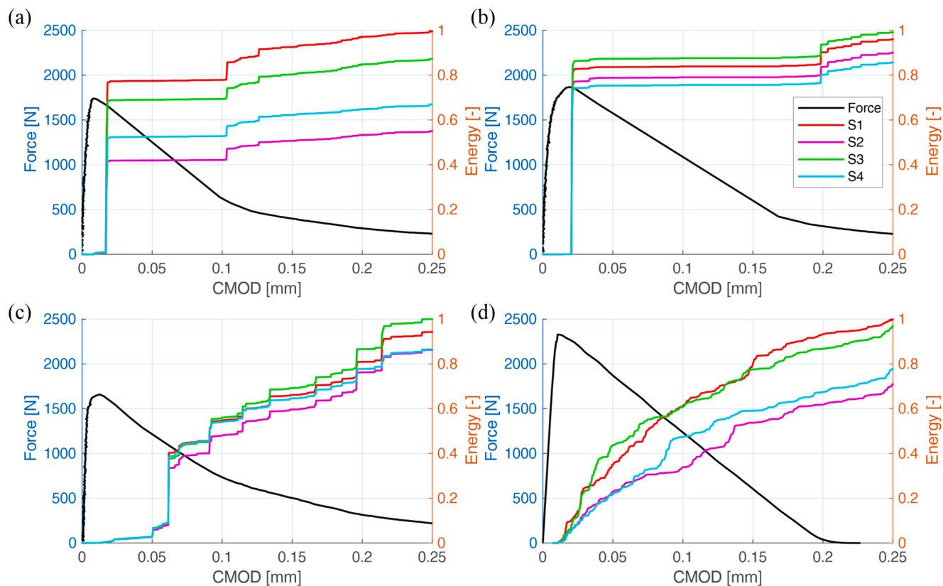
Fig. 10. Cumulative energy curves in the CMOD domain: (a) beam #1, (b) beam #2, (c) beam #3, (d) numerical 3D DEM beam model.
