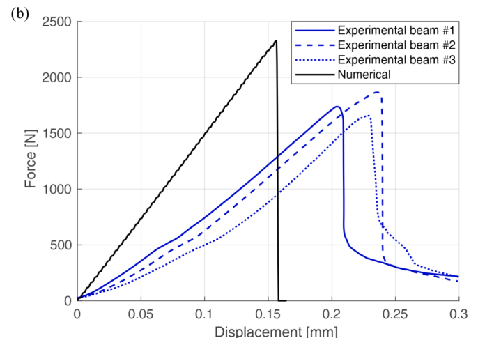
Fig. 4. Results from bending: (a) force-CMOD curves and (b) force-displacement curves for experimental beams #1–3 and numerical beam.
