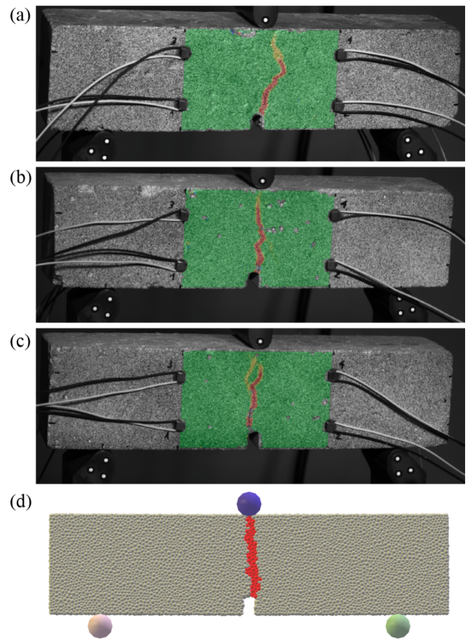
Fig. 5. Final cracking patterns in investigated specimens: (a) beam #1, (b) beam #2, (c) beam #3, (d) numerical 3D DEM beam model.
