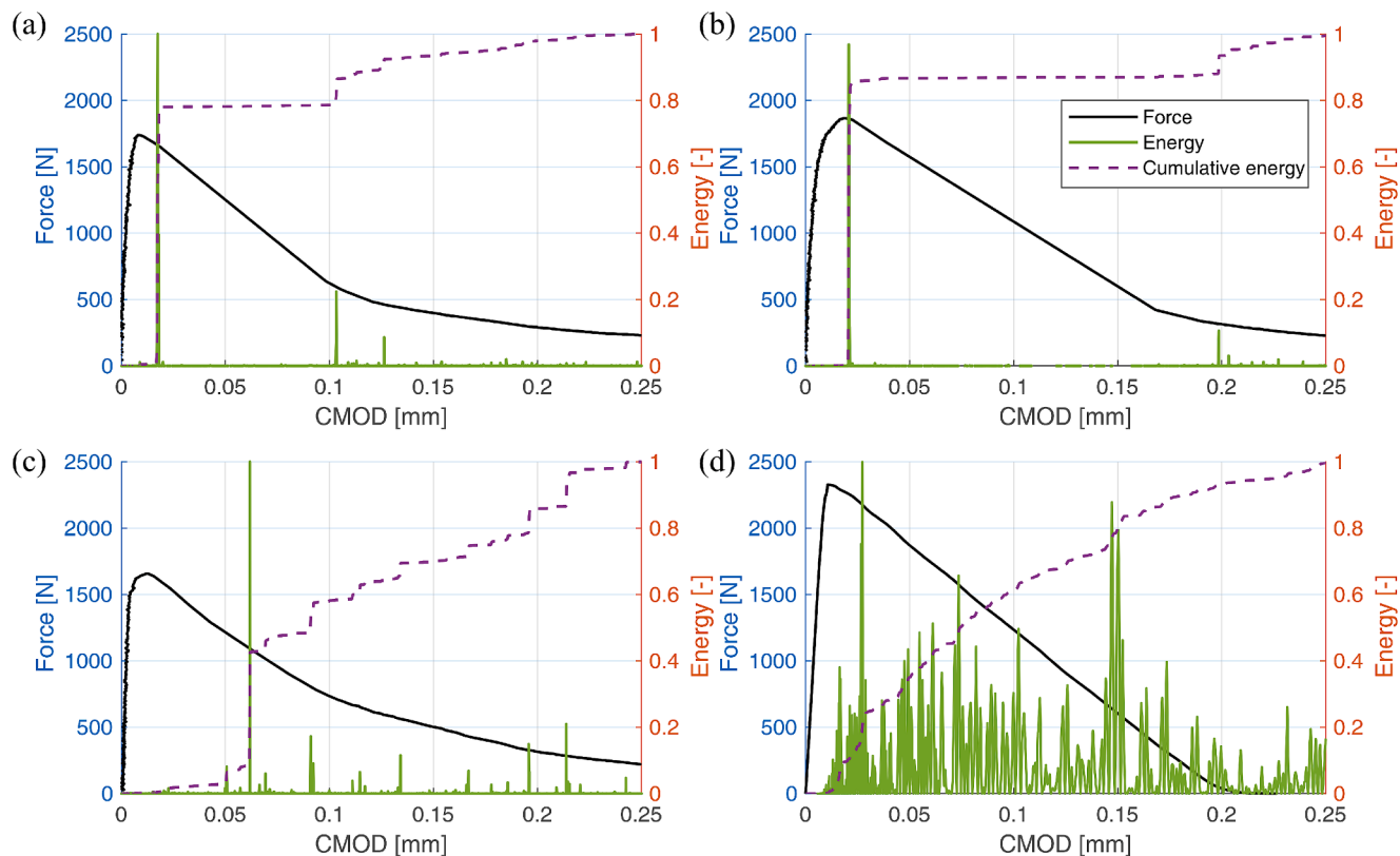
Fig. 9. Energy of signals registered by sensor S1 and the cumulative energy in the CMOD domain: (a) beam #1, (b) beam #2, (c) beam #3, (d) numerical 3D DEM beam model.
