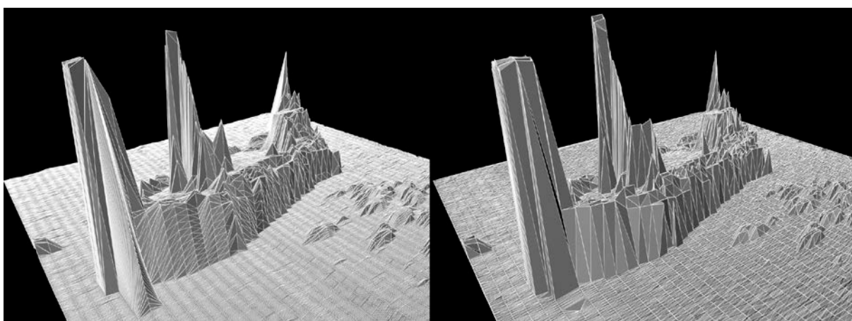
Fig. 4. Comparison of the height-map technique (left) and the 2D Delaunay triangulation (right) of the first dataset.
