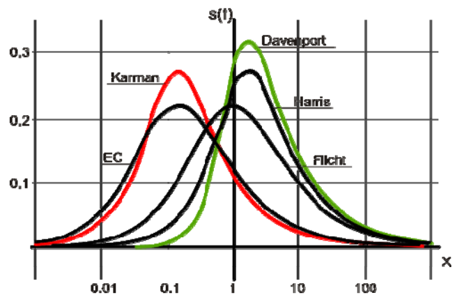
Fig.5. The comparison of the spectrum of wind according to different methods.
