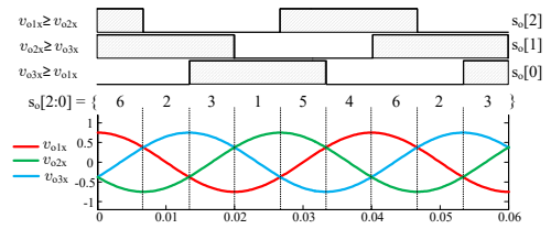
Fig. 6. Identifying the sector of the rotated input vectors using three comparators during an amplitudes asymmetry.
