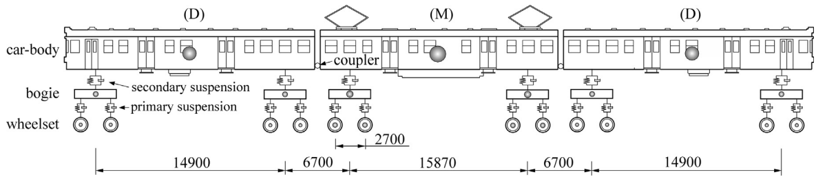
Fig. 2. The mechanical model of the EN57 train in the DMD configuration.
