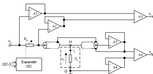
Fig. 5. Simplified schema of the impedance interface for grounded impedance measurement.
