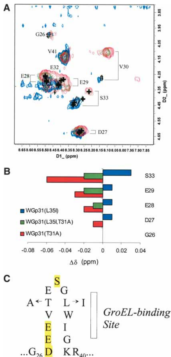
Figure 4. Affects of mutations on the tendency to form \beta -sheet in the most flexible region of the mobile loop. (A) The NH/H^\alpha regions of total correlated (TOCSY) spectra of WGp31(L35I) (blue), WGp31 (black), WGp31(L35I,T31A) (green), and WGp31(T31A) (red). Backbone resonances for residues G34–K39 were not observed, most likely because of dipolar broadening caused by a microsecond–millisecond conformational fluctuation in proximity to the tryptophan side chain. (B) Changes in H^\alpha chemical shift, indicating an increased tendency to adopt \beta -sheet (positive) or decreased tendency to adopt \beta -sheet (negative) in the mobile loops of mutant WGp31 proteins. Nearest-neighbor effects resulting from the T31A substitution confound interpretation of deviations for residues V30–E32. (C) The mobile-loop sequence that forms a nascent \beta -hairpin and binds to GroEL, highlighting the positions used to analyze conformational tendency.
