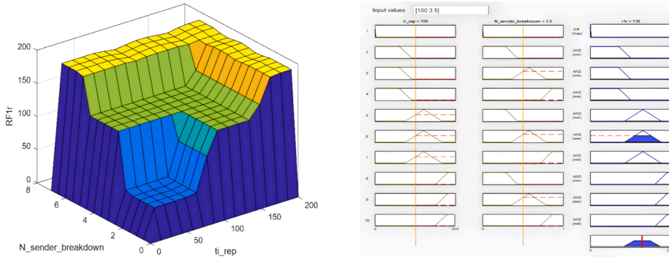
a) Visualization of the logical-linguistic model fuzzy inference RF_1^r – Risk factor associated with the grain loader breakdown b) The rules by which the logical-linguistic model works RF_1^r – risk factor associated with the grain loader breakdown
