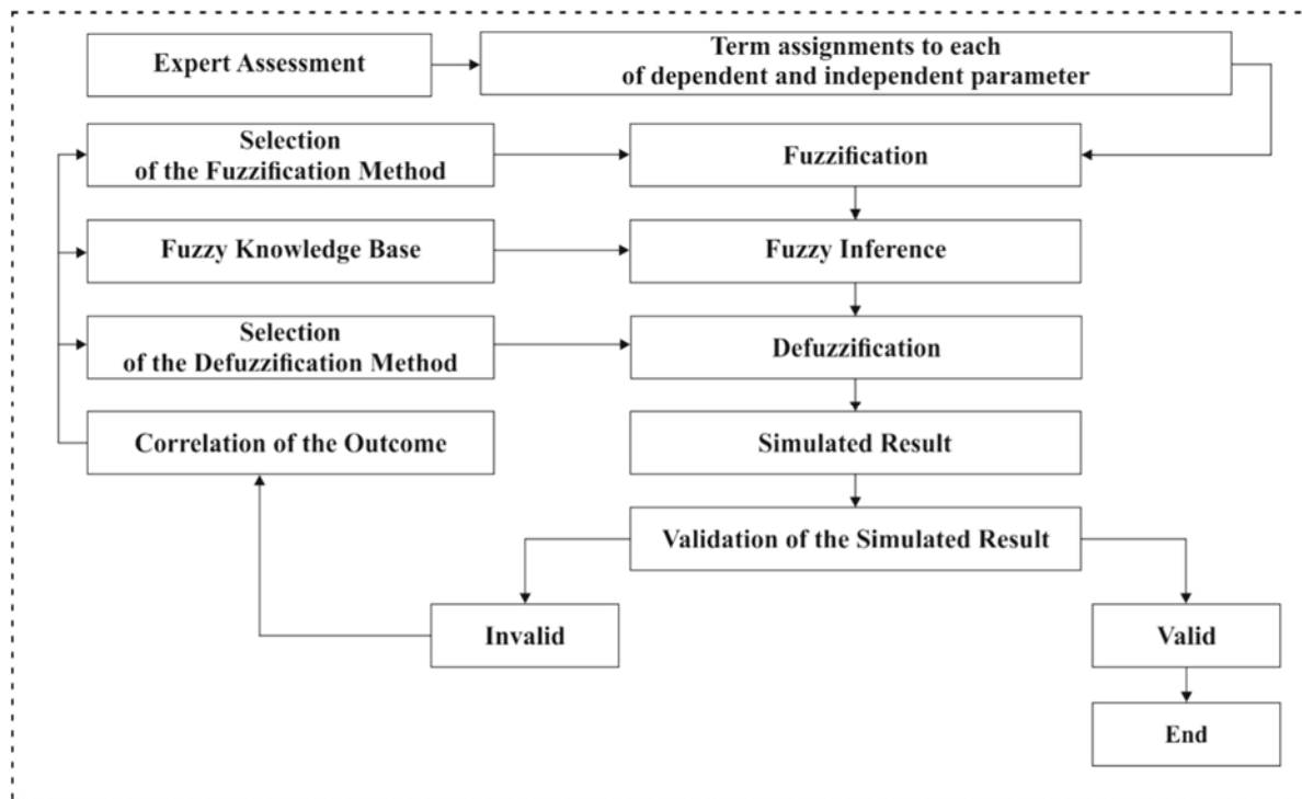
Figure 2. System Parametric Identification Algorithm.
