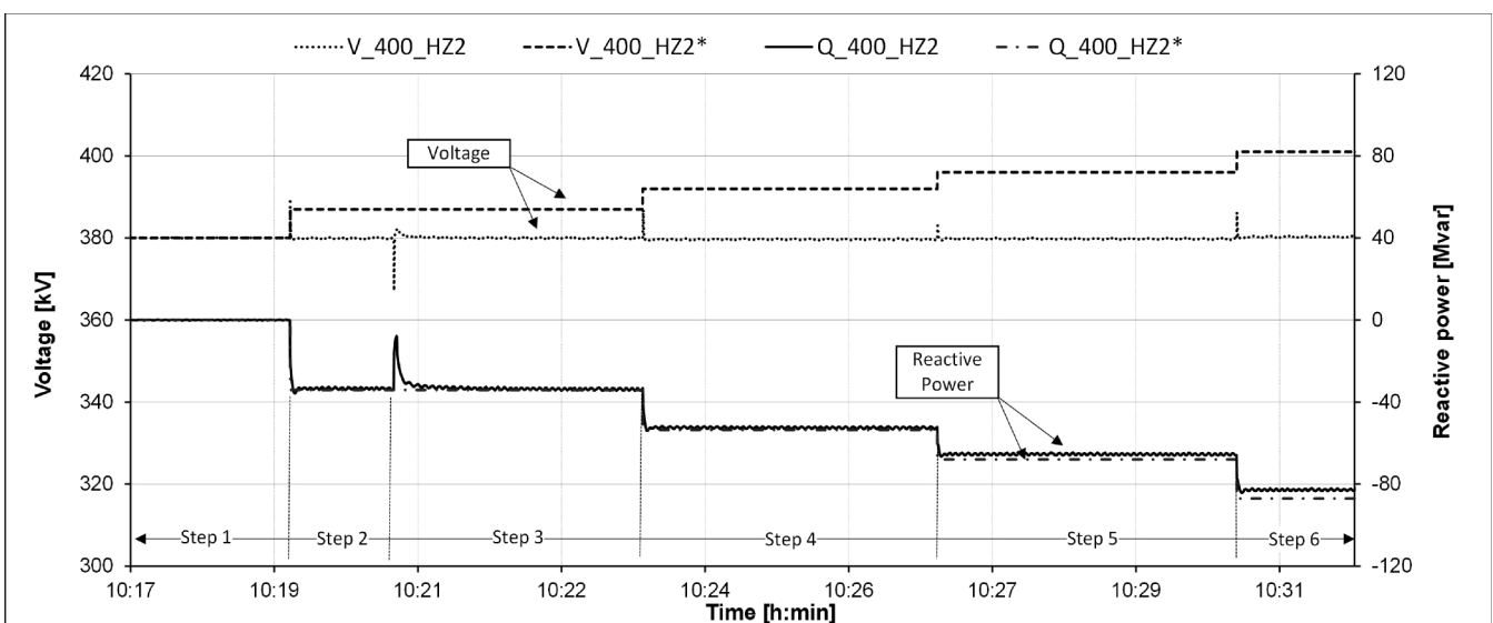
Fig. 8. Voltage and reactive power variation at Zarnowiec node (ZRC) during creation of start-up path (from step 1 to step 6) between Zarnowiec PSP and Kozenice TPP. Mark "*" describes voltage V and reactive power Q levels when load compensation is disabled (classic assumption – results of simulation).
