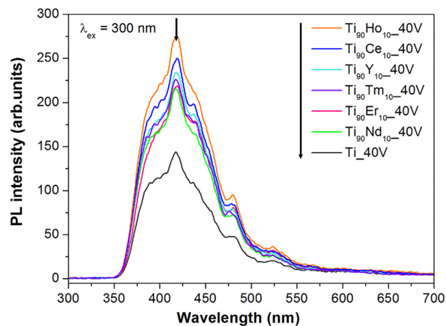
Fig. 5. Photoluminescence spectra of \text{TiO}_2 and RE-modified \text{TiO}_2 nanotubes.
