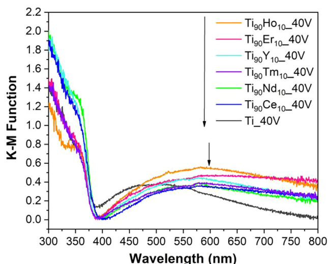
Fig. 4. UV-Vis Kubelka-Munk absorption of \text{TiO}_2 and RE-modified \text{TiO}_2 nanotubes.
