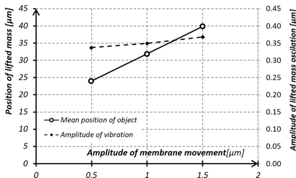
Fig. 7. Mean position ( h_{\text{Top}} ) and the amplitude of vibration of the modelled object as a function of amplitude of membrane movement
