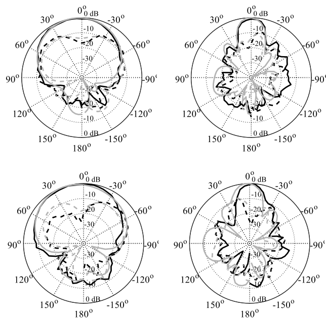
Fig. 8. Simulated (gray) and measured (black) xz - (left) and yz -plane (right) patterns for 27.5 GHz, and 29.0 GHz (from top to bottom); co-pol (—), cross-pol (- -).
