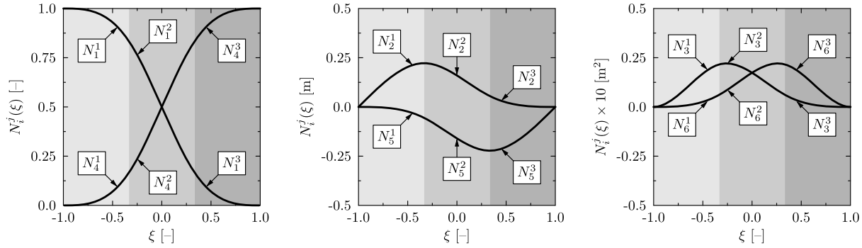
Fig. 2. Piecewise 1-D spline-based elemental shape functions N_i^j(\xi) of degree p=3 , associated with nodal DOFs: displacements q_1 and q_2 (left), rotations q'_1 and q'_2 (middle), rotation derivatives q''_1 and q''_2 (right), in the local normalised co-ordinate system of the element \xi , obtained in the case of the unit element length l=1 m.
