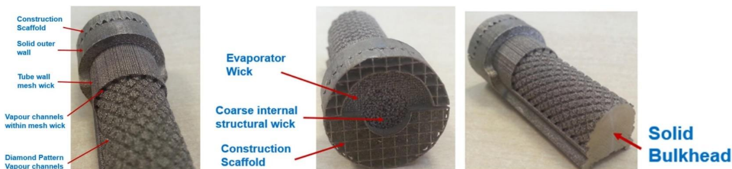
Figure 10. AM LHP evaporator [17].
