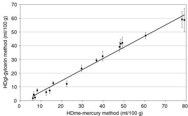
FIGURE 5. Comparison of the diffusible hydrogen content obtained with the mercury method and glycerin method in the up to 80 ml/100 g range.
