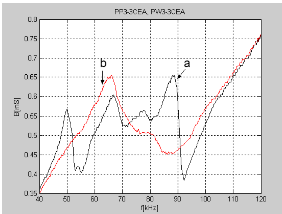
Fig.7. Susceptance of transducer in: a) - air, b) - water
