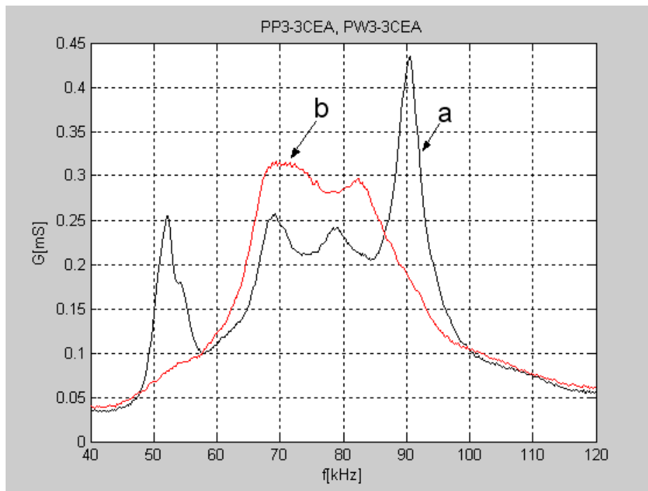
Fig.6. Conductance of transducer in: a) - air, b) - water
