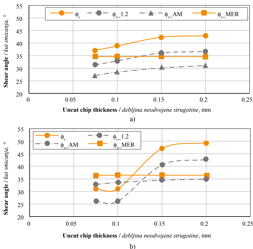
Figure 4 Shear angles \Phi_c while cutting on sliding microtome in longitudinal direction to pine wood fibres for MC = 12\% (a) and MC = 20\% (b) in a function of uncut chip thickness h . Legend: \phi_c – shear angle determined in a function of chip compression ratio \lambda_h , \phi_{c\_1.2} – shear angle computed in a function of chip compression ratio \lambda_h while measured chip thickness h_{ch} was enlarged by 20 %, \phi_{c\_AM} – shear angle obtained from Atkins model, \phi_{c\_MER} – shear angle calculated with Merchant model Slika 4. Kutovi smicanja \Phi_c tijekom rezanja na kliznome mikrotomu u smjeru vlaknaca borovine pri (a) MC = 12\% i (b) MC = 20\% u funkciji debljine neodvojene strugotine h ( \phi_c – kut smicanja određen u funkciji omjera kompresije strugotine \lambda_h , \phi_{c\_1.2} – kut smicanja izračunan u funkciji omjera kompresije strugotine \lambda_h , a izmjerena debljina strugotine h_{ch} povećana je za 20 %, \phi_{c\_AM} – kut smicanja dobiven iz Atkinsova modela, \phi_{c\_MER} – kut smicanja izračunan prema Merchantovu modelu)
