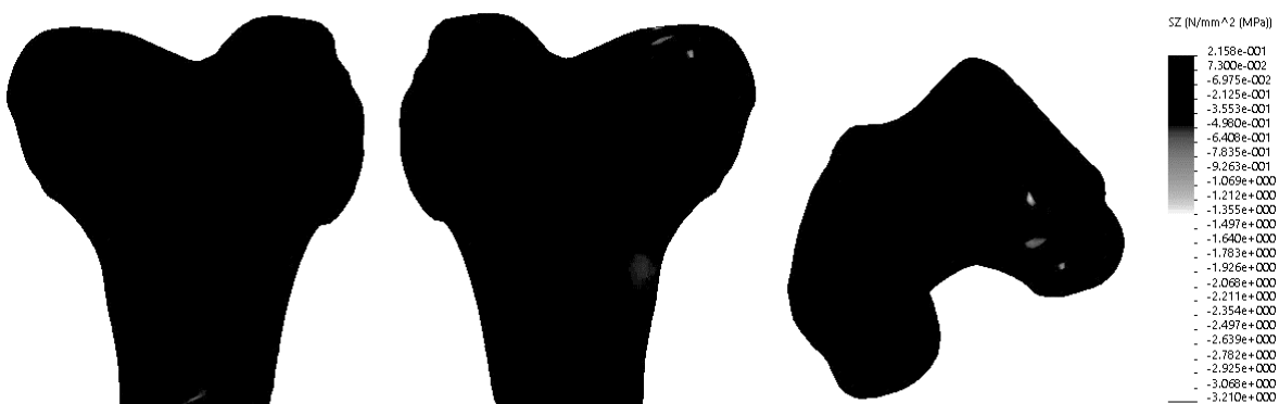
Fig. 11. Normal stresses along the Z axis (mechanical knee axis) of the proximal tibia (both materials – bone)
