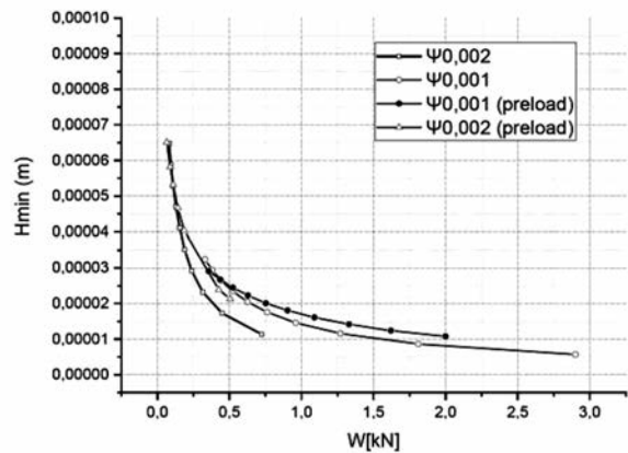
Fig. 8. Comparison of minimum water film thickness of bearing No. 1 (cylindrical) and No. 2 (three-surface preloaded) as function of acting load for two variants of relative clearance value - 0.001 and 0.002. Load directed towards axial groove (between segments)
