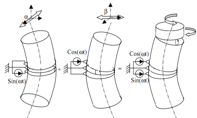
Fig. 1. Operation principle of a rotation mode motor [4]
