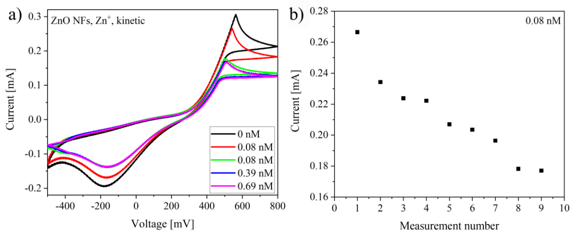
Fig. 4.37 a) CV response of the ZnO NFs electrode in \text{K}_4[\text{Fe}(\text{CN})_6] PBS electrolyte with different concentration of zinc ions. b) Change of current at the oxidations peak in the presence of 0.08 nM of \text{Zn}^{2+} .
