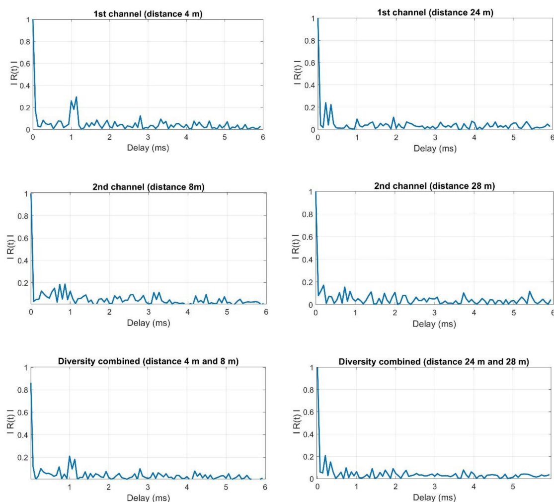
Figure 11. Example of the estimates of the impulse response moduli obtained during the tests in real conditions.
