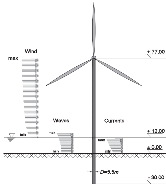
Fig. 4. Environmental loads
