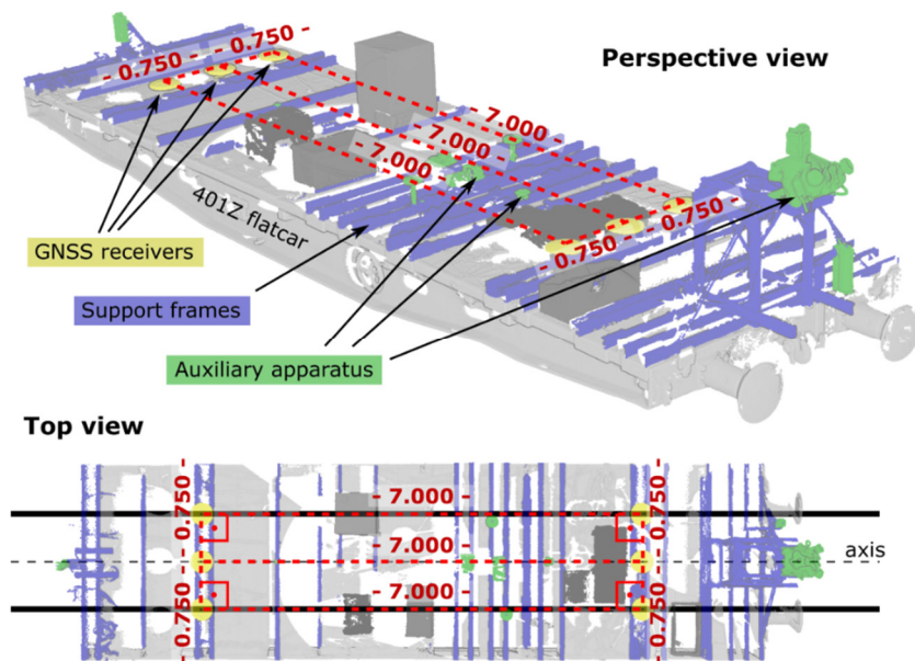
Figure 1. Configuration of six GNSS receivers on the railway platform.
