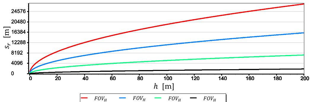
Figure 5. Horizon sagitta s_r as a function of the height of the camera a.s.l. h (for FOV_H equals 30°, 60°, 90° and 120°, R = 6,378,000.0 m, k = 0.16 ).
