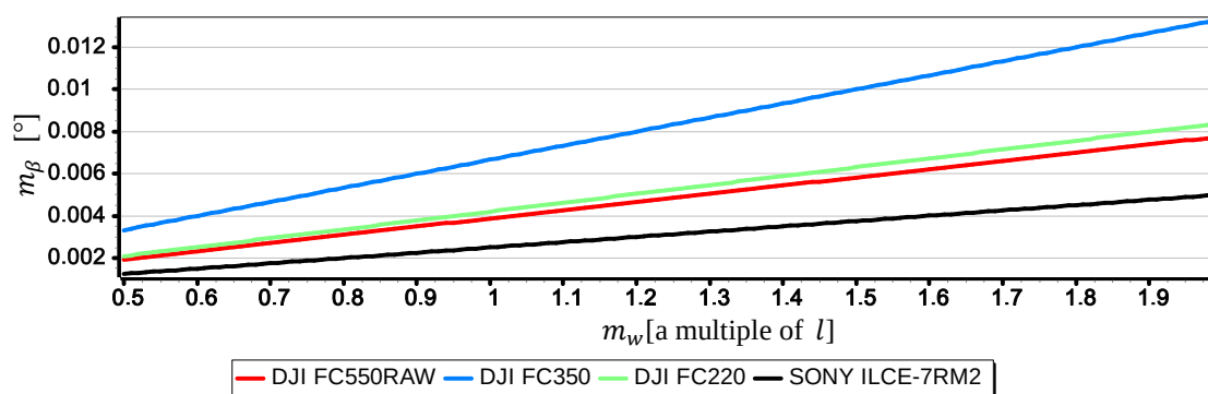
Figure 23. Mean error of measurement m_\beta as a function of m_w for \beta = 15^\circ (only the second component of the Formula (3) was used in the calculations).
