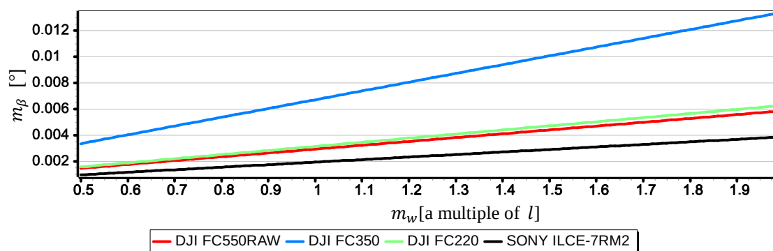
Figure 22. Mean error of measurement m_\beta as a function of m_w for \beta = 10^\circ (only the second component of the Formula (3) was used in the calculations).
