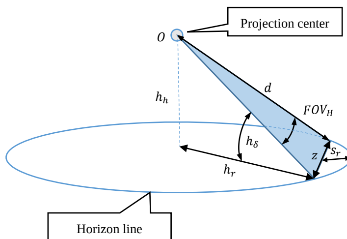
Figure 4. Part of the horizon line (with the length z ) in the FOV_H of the camera.
