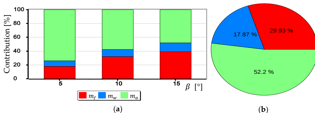
Figure 27. Percentage contribution for SONY ILCE-7RM2 camera: (a) Calculated for \beta equals 5^\circ, 10^\circ and 15^\circ ; (b) Calculated as a mean value.
