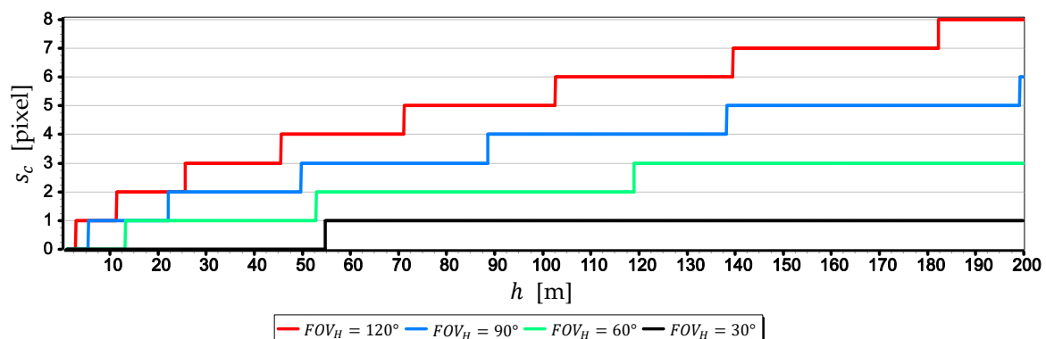
Figure 6. Horizon sagitta s_c as a function of the height of the camera a.s.l. h (for FOV_H equals 30°, 60°, 90° and 120°, R = 6,378,000.0 m, k = 0.16 , p_H = 4000 pixels).
