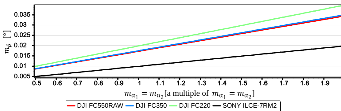
Figure 24. Mean error of measurement m_\beta as a function of m_{\alpha_1} = m_{\alpha_2} for \beta = 5^\circ (only the last two components of the Formula (3) were used in the calculations).
