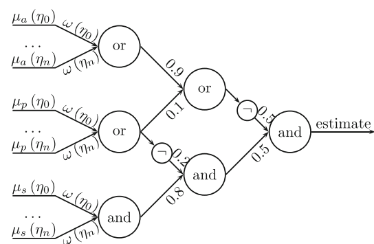
Fig. 5 Fuzzy neural network estimating the suitability of reactions based on the actual state of needs and the simulated effects of reactions [19]: the inputs of neurons are (from the bottom) the values of the membership functions of satisfaction, prealarm and alarm for all the considered needs; the importance of the needs is underscored by using their individual weights/weighting functions \eta_i ; the output of the network is an estimate \hat{if} of the impact (factor) of a given reaction on the state of the needs \eta_0 through \eta_n
