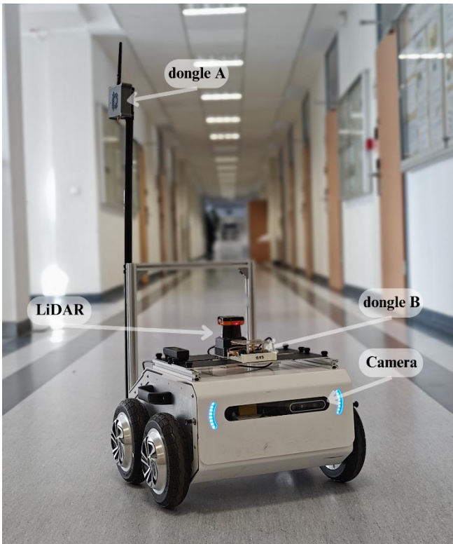
Fig. 1. Measurement robot in indoor environment
