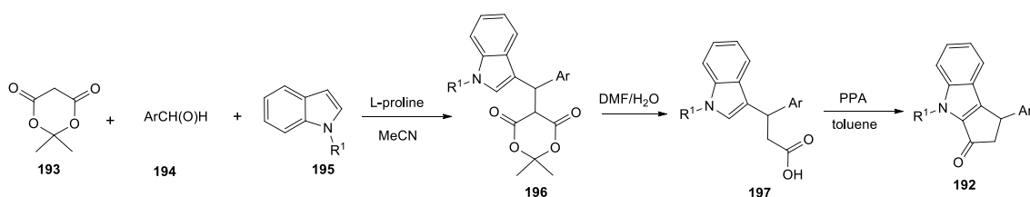
Figure 66 Preparation of 1-aryl-1,2-dihydrocyclopenta[b]indol-3(4 H )-ones
