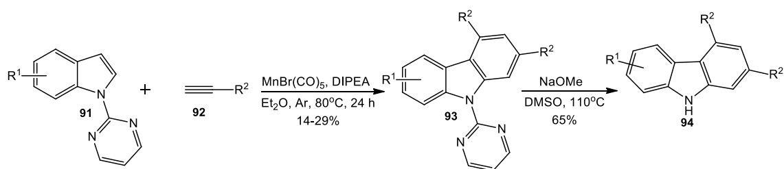
Figure 47 MnBr(CO) 5 -catalyzed synthesis of carbazole derivatives
