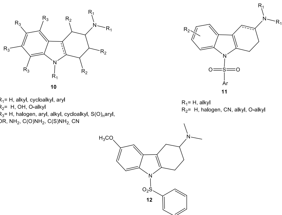
Figure 11 5-HT 6 receptor ligands
