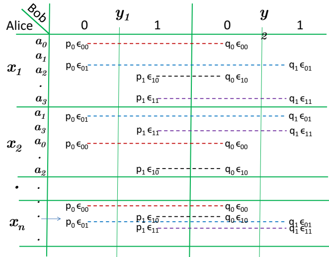
FIG. 3. (Color online) The box \{p(a, b|x, y)\} of Alice and Bob. Dashed lines represent which pairs give rise to confused outcomes (a_i 's) and their lower bounds. Note that, for some choice of inputs (x, y) , some or all confused outcomes (a_i 's) may coincide with each other.
