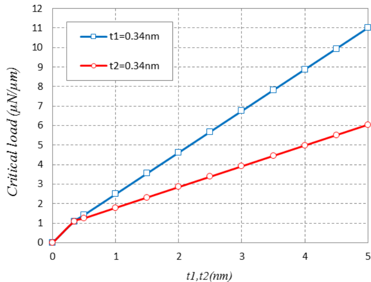
Fig. 10. Variation of the core thickness versus the face thickness ( l=h , L_x=15h , \eta=1 , k_1=k_2=1 , SSSS, Epoxy)
