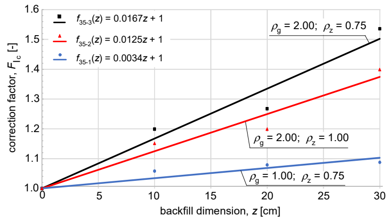
Figure 13. Value of the correction factor ( F_{Ic} ) as a function of the stabilized backfill dimension ( z ) and its thermal parameters for a power cable line with a cross-sectional area of 35 \text{ mm}^2 .
