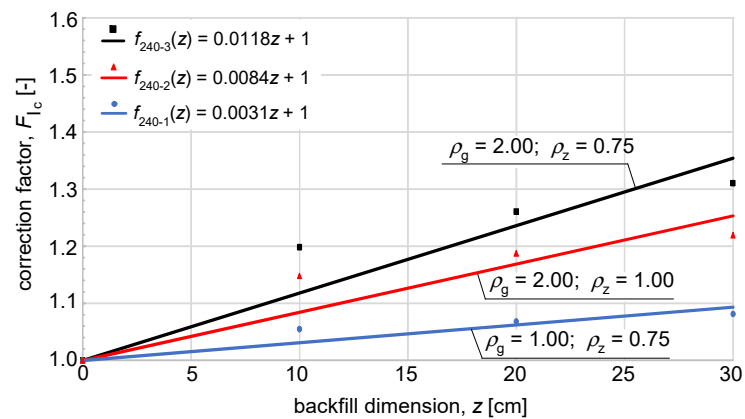
Figure 15. Value of the correction factor ( F_{Ic} ) as a function of the stabilized backfill dimension ( z ) and its thermal parameters for a power cable line with a cross-sectional area of 240 \text{ mm}^2 .
