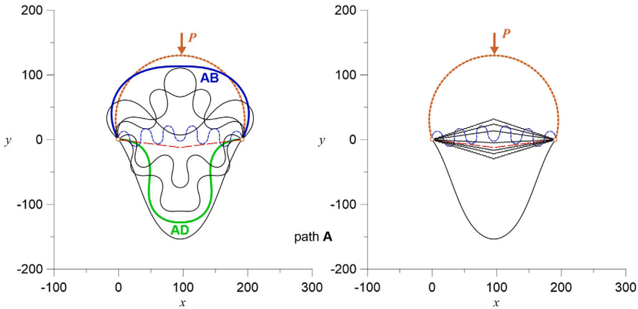
Fig. 9. Selected arch configurations calculated with 72e4 C^0 elements.
