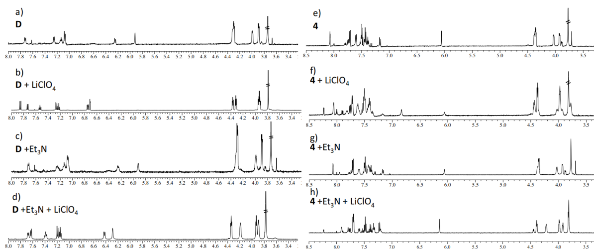
Fig. 9. Comparison of ^1\text{H} NMR spectra of 16-membered hydroxyazobenzocrowns D (left) and 4 (right) and spectra registered in the presence of lithium perchlorate; triethylamine and triethylamine and lithium perchlorate in acetonitrile- d_6 .
