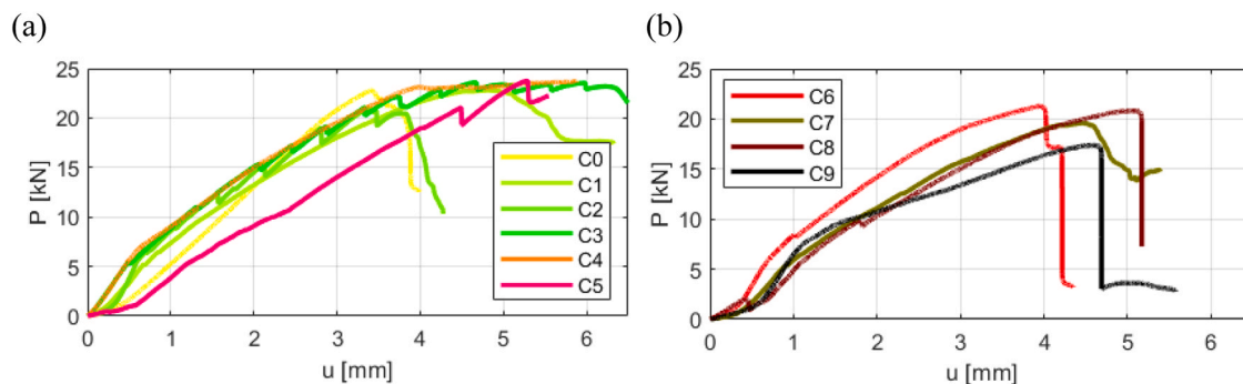
Fig. 12. Force-displacement function while three-point bending tests for specimens: (a) C0-C5, (b) C6-C9.
