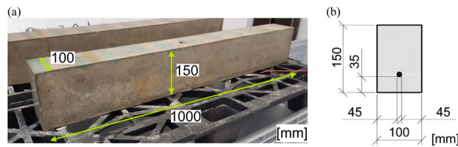
Fig. 2. Beam specimen: (a) overall view, (b) cross-section.
