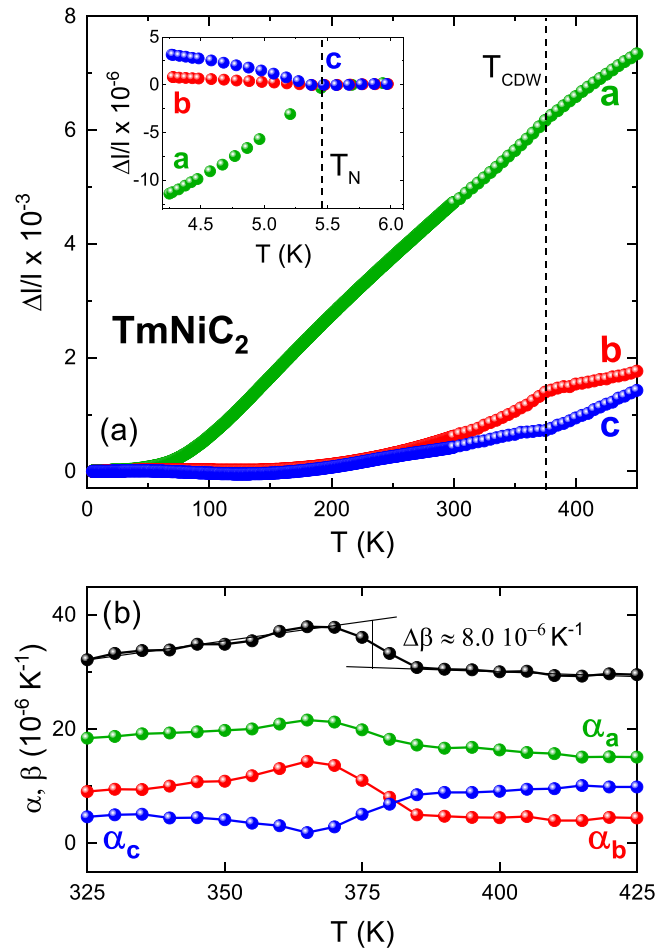
FIG. 2. (a) Temperature-dependent thermal expansion along orthorhombic a (green), b (red), and c (blue) orientations of \text{TmNiC}_2 . Inset zooms towards the AF transition. Both, CDW and AF transition temperatures are indicated by dotted lines; (b) thermal expansion coefficients and volume expansion coefficient vs temperature. Solid lines are a guide to the eye.
