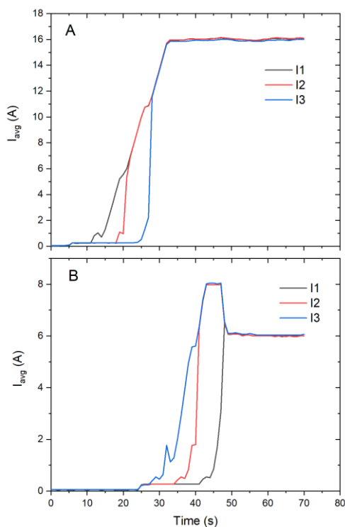
Fig. 1. Changes in current drawn from the mains after starting the charging process in the EV in the case of charging point no. 1 (A) and no. 2 (B)
