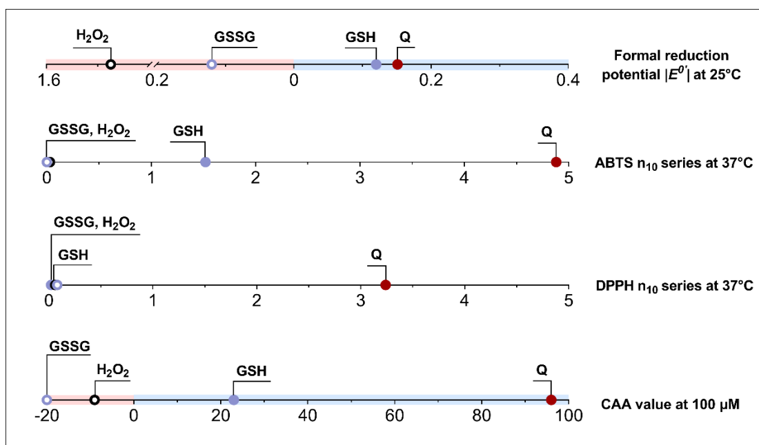
Figure 4.30. Axes comparing redox properties of endogenous pro-oxidants ordered according to: formal reduction potential ( E^{\circ'} [V], shown as absolute values); n_{10} values calculated based on ABTS or DPPH tests; the cellular antioxidant activity (CAA) values measured in cells cultured in complete medium and treated with 100 \mu\text{M} concentration of investigated compounds (GSH, glutathione; GSSG, glutathione disulphide; \text{H}_2\text{O}_2 , hydrogen peroxide; Q, quercetin). Colour highlights along axes mark reducing (blue) and oxidizing (red) ranges of compounds' activity.
