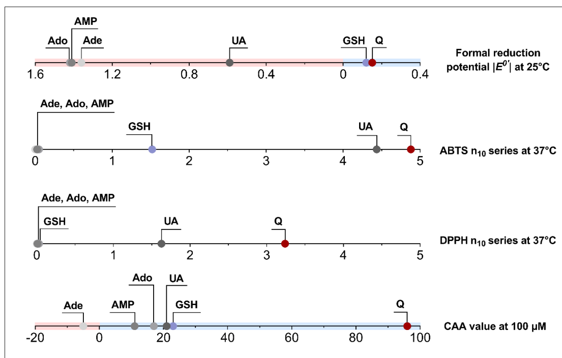
Figure 4.16. Axes comparing redox properties of purine derivatives ordered according to: formal reduction potential ( E^{0'} [V], shown as absolute values); n_{10} values calculated based on ABTS or DPPH tests; the cellular antioxidant activity (CAA) values measured in cells cultured in complete medium and treated with 100 \mu M concentration of investigated compounds (Ade, adenine; Ado, adenosine; AMP, adenine-5'-monophosphate; GSH, glutathione; Q, quercetin; UA, uric acid). Colour highlights along axes mark reducing (blue) and oxidizing (red) ranges of compounds' activity.
