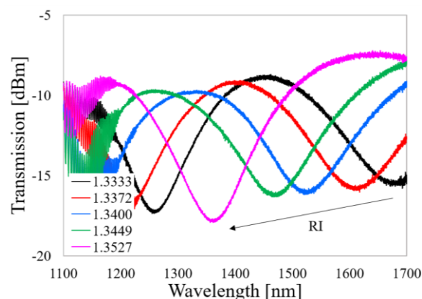
Figure 4. Spectral response of the reference \mu IMZI with cavity diameter d = 60 \mu\text{m} . An arrow indicates the shift of the minimum with RI.
