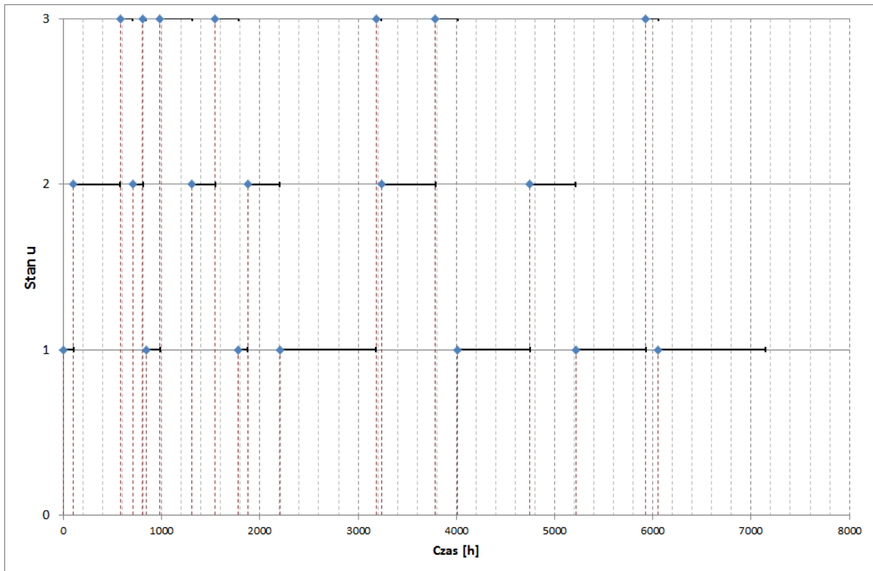
Fig. 4 The states-transitions graph of the of the process \{W'(t): t \in T\} . u_1 – full serviceability state.
