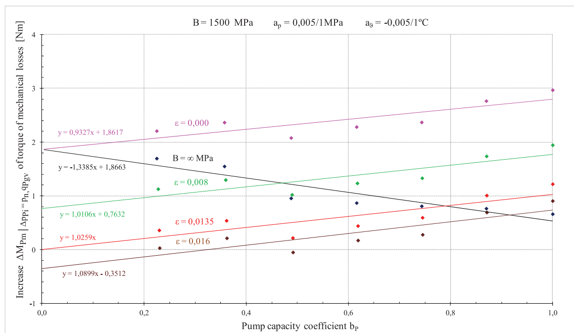
Fig. 6 Picture of the relations of increase \Delta M_{Pm} |_{\Delta p_{pi} = 32 MPa; q_{pgv}} of torque of mechanical losses in the pump „working chambers - shaft” assembly (pump HYDROMATIK A7V.58.DR.1.R.P.F.00 type) to the geometrical working capacity q_{pgv} ( b_p coefficient) with assumed values of modulus B of hydraulic oil elasticity and oil aeration coefficient \epsilon [10, 11]
