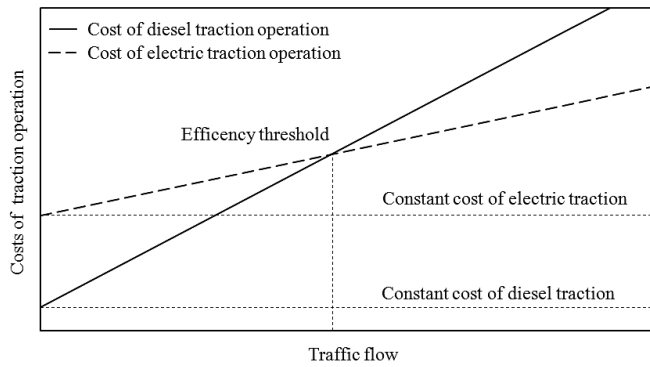
Fig. 1. Threshold of economic efficiency between usage of diesel and electric traction in function of traffic flow
