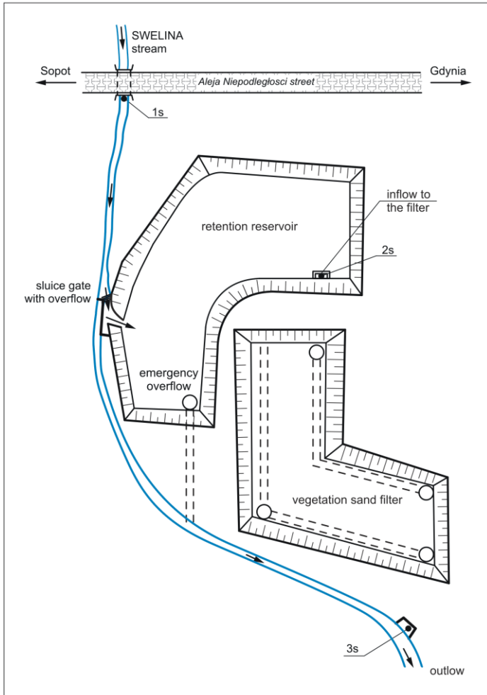
Fig. 3. The CW system on Swelina Stream, according to [11]
