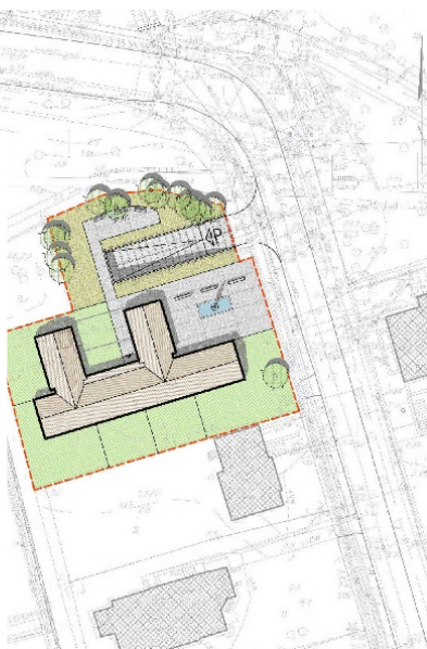
III. 3. Multi-family residential and public utility building in Sopot at Powstańców Warszawy Street: a) site plan, b) perspective, source: Fort Taraszkiewicz Architekci. http://www.fort-taraszkiewicz.pl/ (accessed: 20.02.2023)
