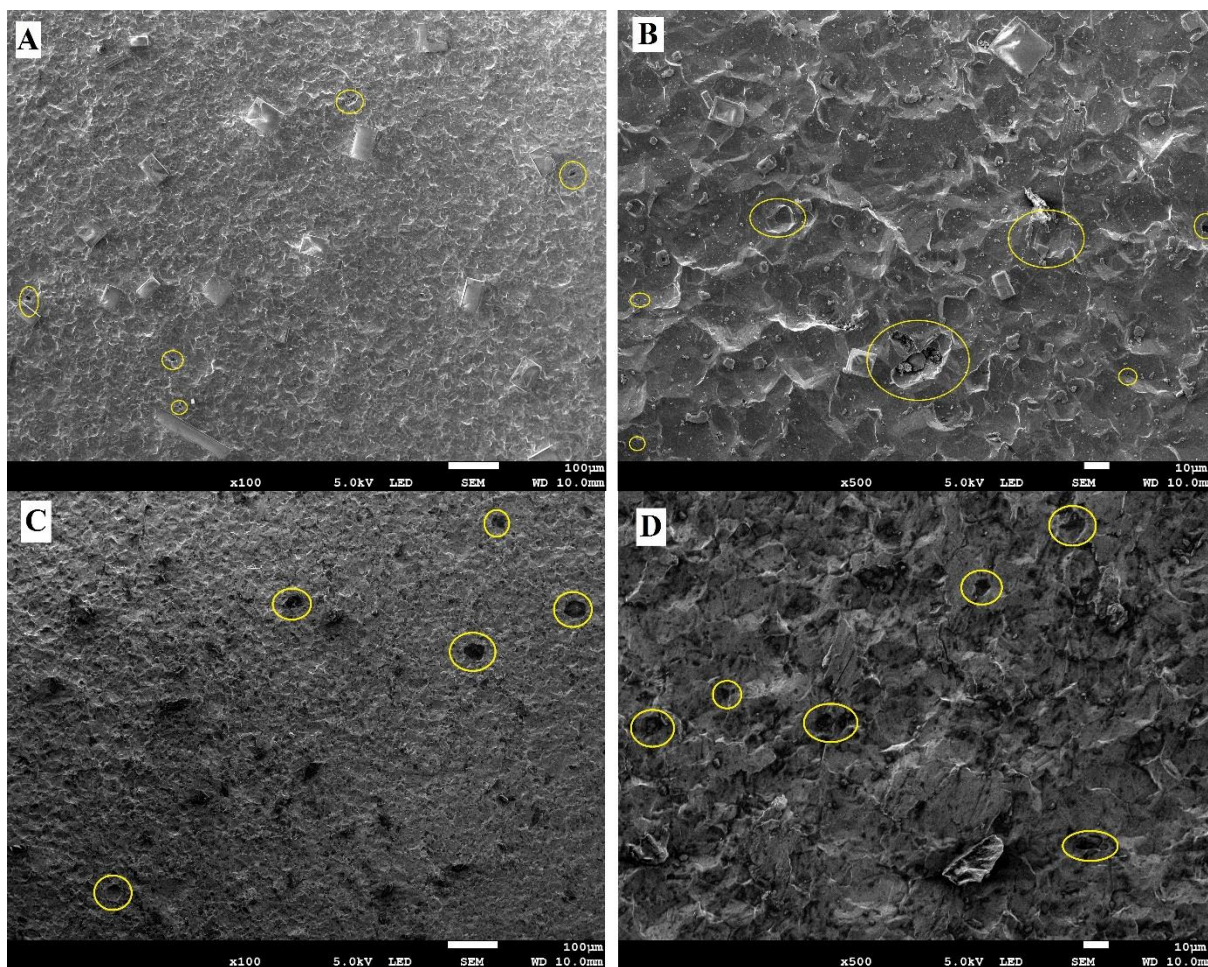
Fig. 7. Topography of the surface of titanium after the corrosion test (Ringer's solution: 100x – A and 500x – B, Artificial Saliva solution: 100x – C and 500x – D, yellow circles – micropores/craters)
