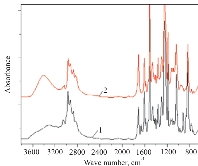
Fig. 2. IR-spectra of blend III: 1 – after mixing all components, 2 – after curing for 24 h at room temperature with further gradual heating at 383 (0.5 h), 403 (0.5 h) and 423 K (0.5 h)
