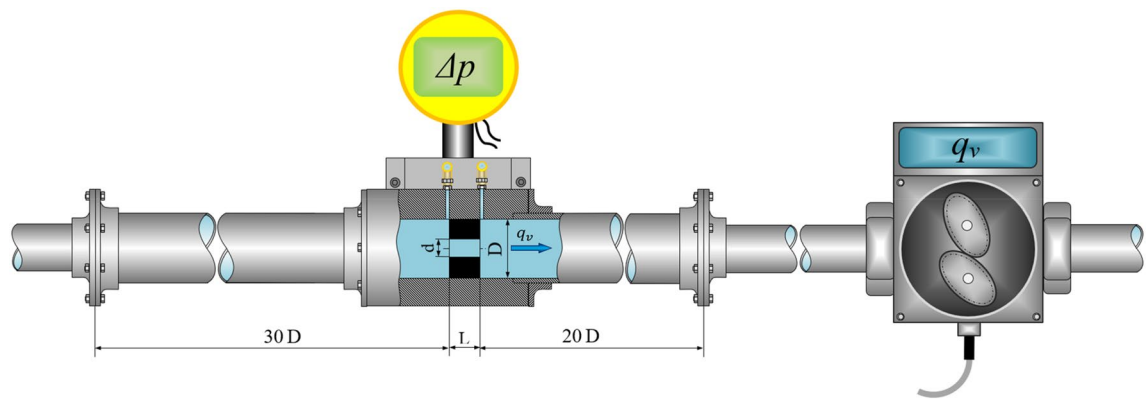
Figure 2. Schematic of the hydraulic measuring system.
